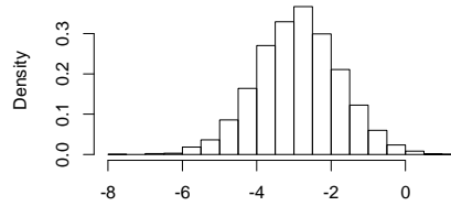
Histogram of log 10 (intake)
