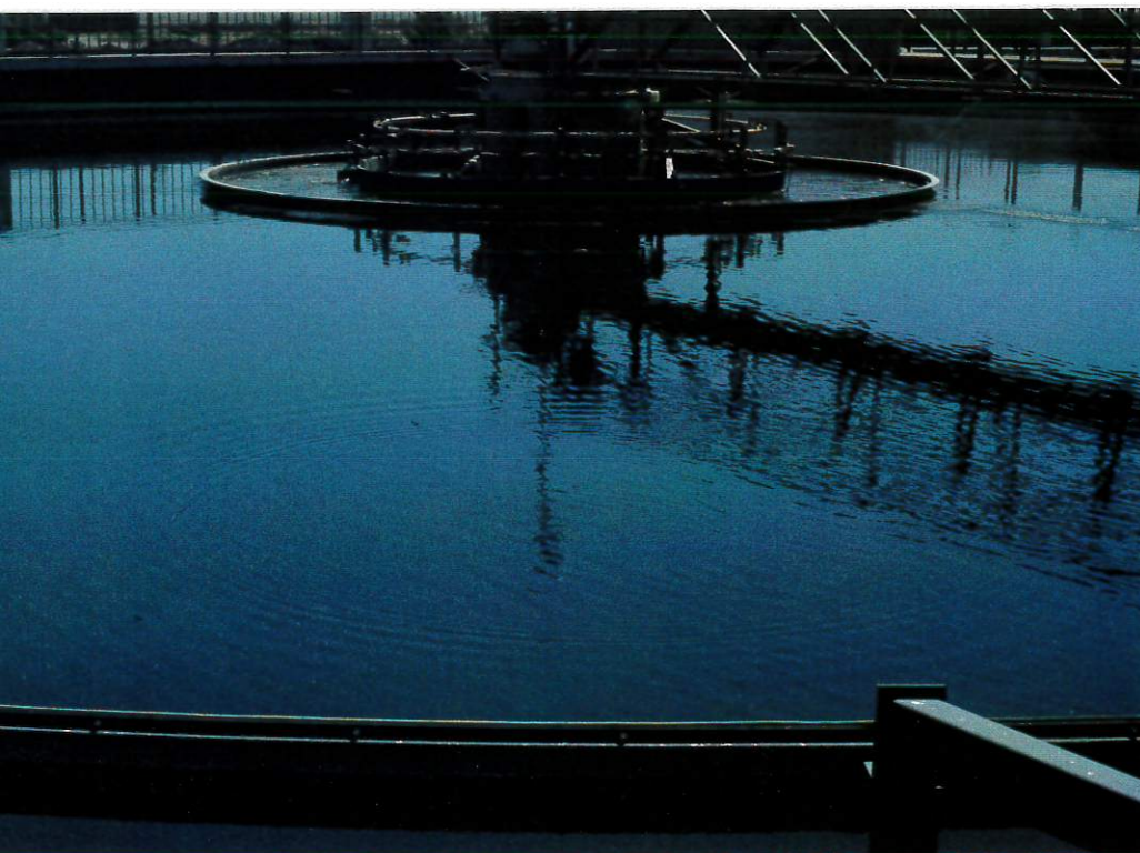
A secondary clarifier in which sludge settles before effluent undergoes dual-media filtration.
